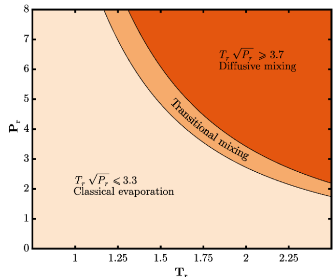
Figure 1. Classification of the mixing regimes observed in [1]. Both P_r and T_r are calculated by dividing the imposed far-field pressure and temperature ( P_g, T_g ) by the critical values of the fuel ( P_c, T_c ). In the classical evaporation domain droplets remain spherical throughout their lifetime. In the transitional mixing regime there is evidence of surface tension but significant droplet stretching and deformation, leading to an accelerated mixing. In the diffusive mixing domain some surface tension may be observed initially but droplets rapidly transition to a mixing regime dominated by diffusion, with no more evidence of surface tension.
